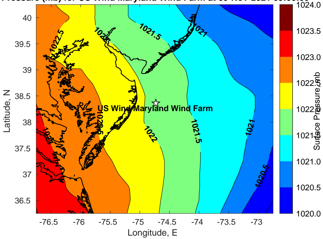
Surface Pressure (mb) for US Wind Maryland Wind Farm at 09-Nov-2021 09:00:00
